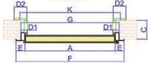
İTALYAN KASA ITALIAN FRAME
