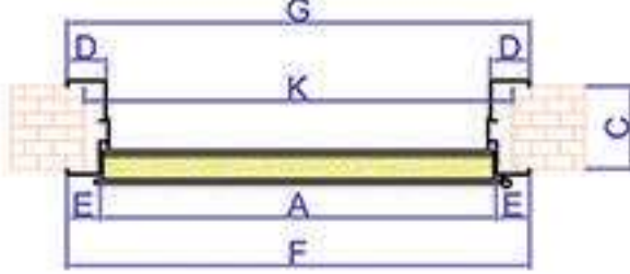
AYARLI KASA ADJUSTABLE FRAME
