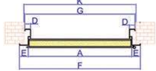
SABİT KASA FIX FRAME
